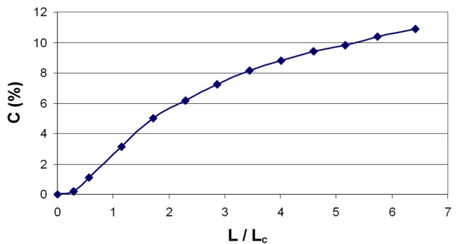
Fig. 8 Difference between the maximum contact pressures obtained assuming an E_EP and EP_EP behavior versus the dimensionless load L/L_c
