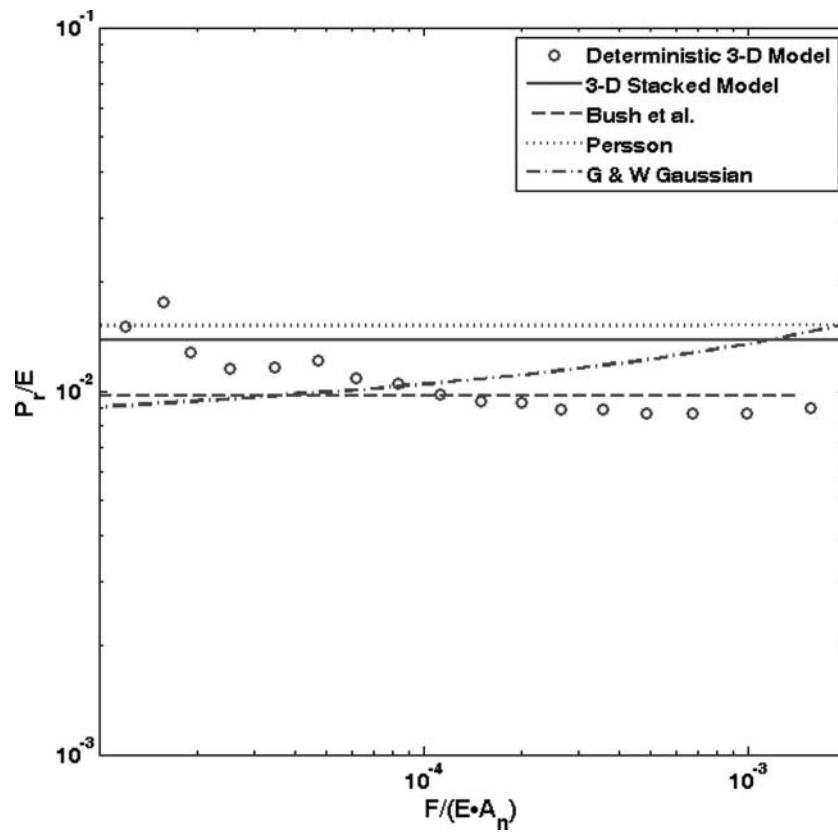
Fig. 4—Resulting model predictions of normalized real contact pressure versus normalized load for a 100 × 100 course mesh of surface 1.
