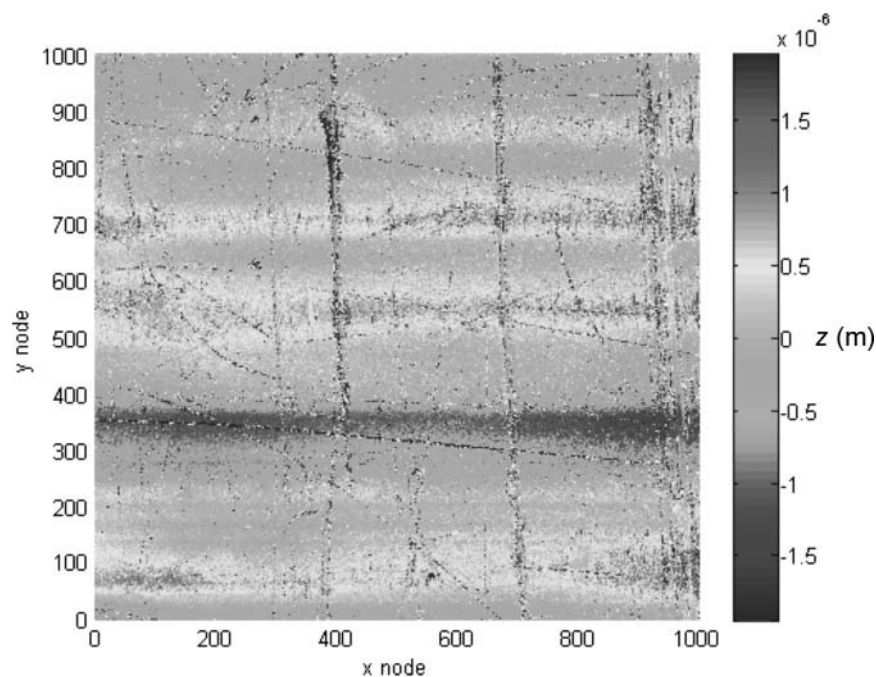
Fig. 7—Measured profile of surface 2.
