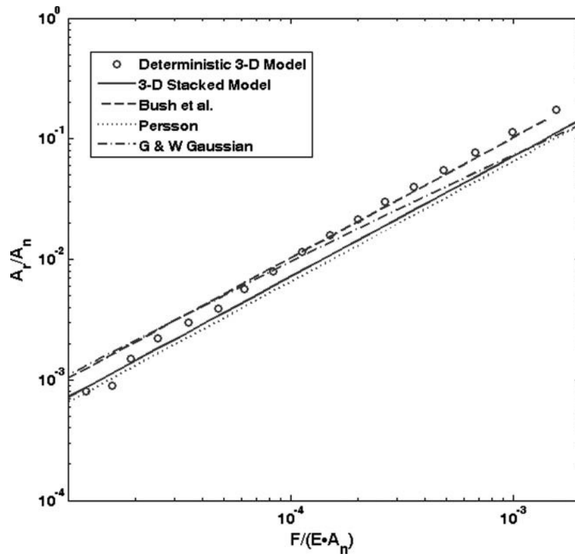
Fig. 3—Resulting model predictions of normalized real contact area versus normalized load for a 100 × 100 course mesh of surface 1.
